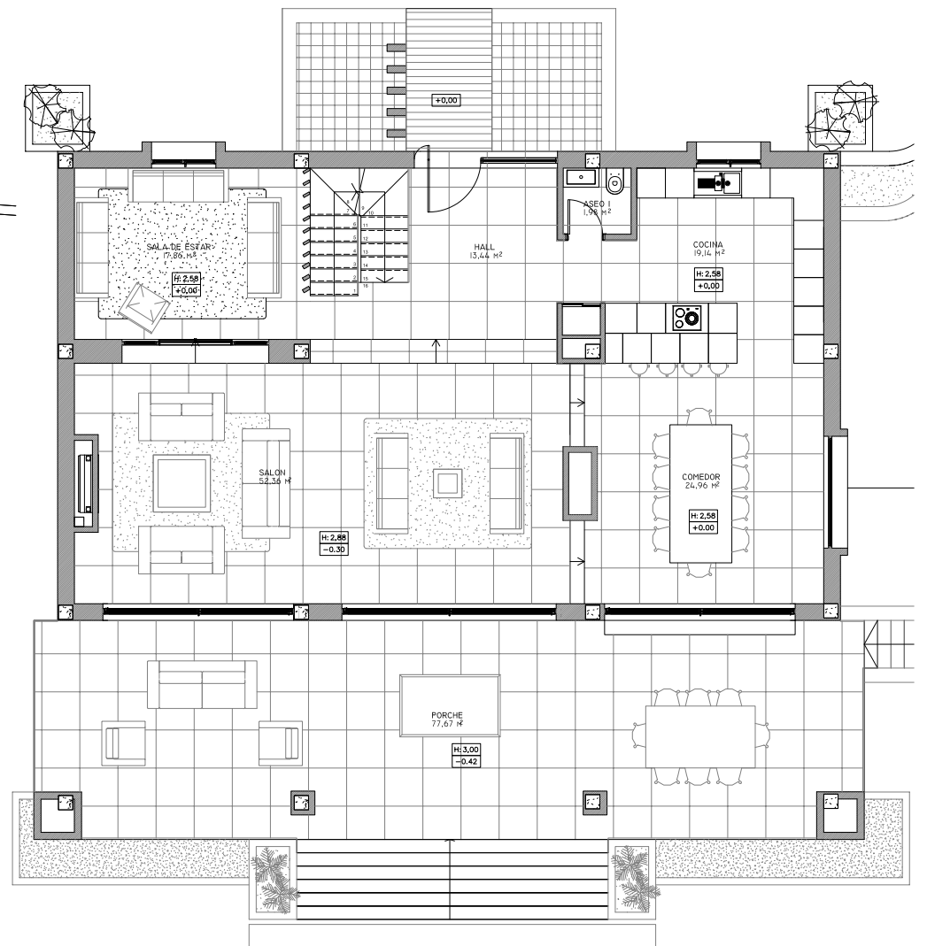
PLANTA BAJA GROUND FLOOR
